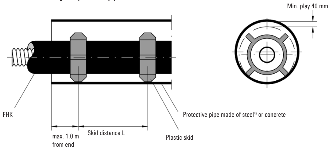
Figure 2: Installing FHK through straight-running protective pipes without offset, using skids. Max. length of protective pipe \geq 50 m 1)
