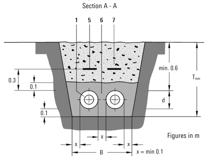
Figure 2: Cross-section of trench
