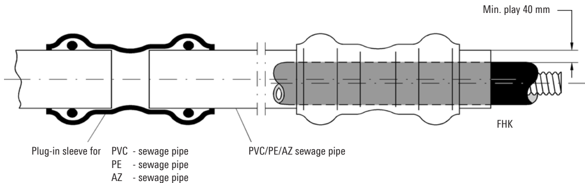
Figure 1: Installing FHK through straight-running protective pipes without offset, not using skids. Max. length of protective pipe \geq 50 m 1)
